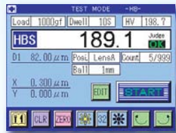
Light-load brinell mode
